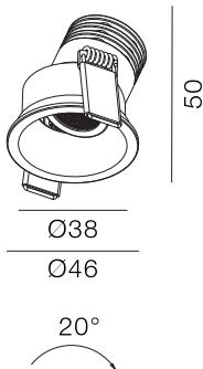
DL6022 IP44
